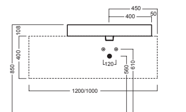
SLIDING wood system _taglio 2 dx - cut 2 rh
